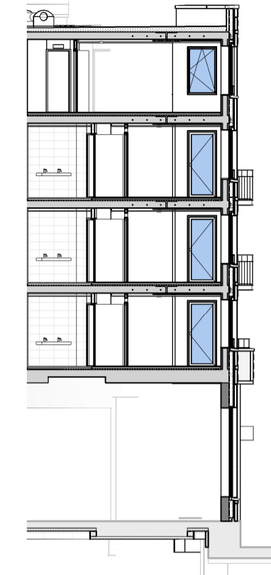
doorsnede pand F (fragment A)
