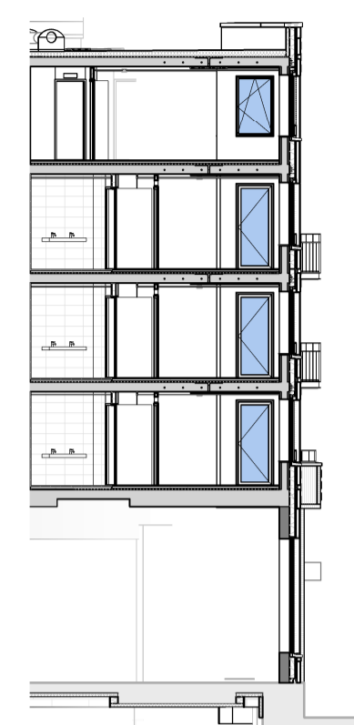
doorsnede pand F (fragment A)
