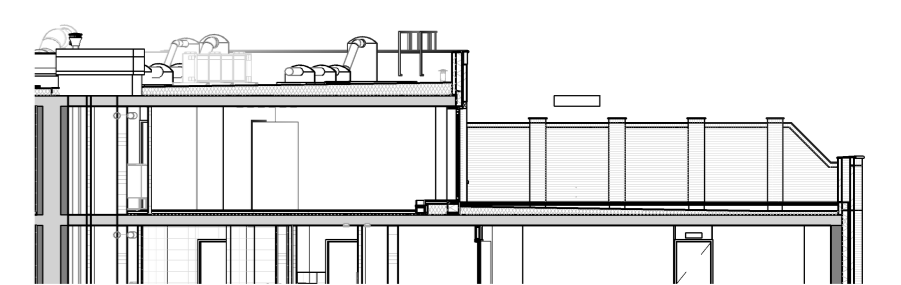
fragment pand H (boven I) schaal 1:200
