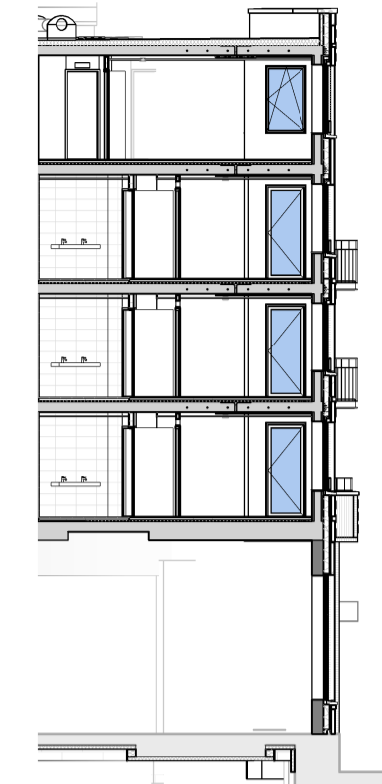
doorsnede pand F (fragment A)
